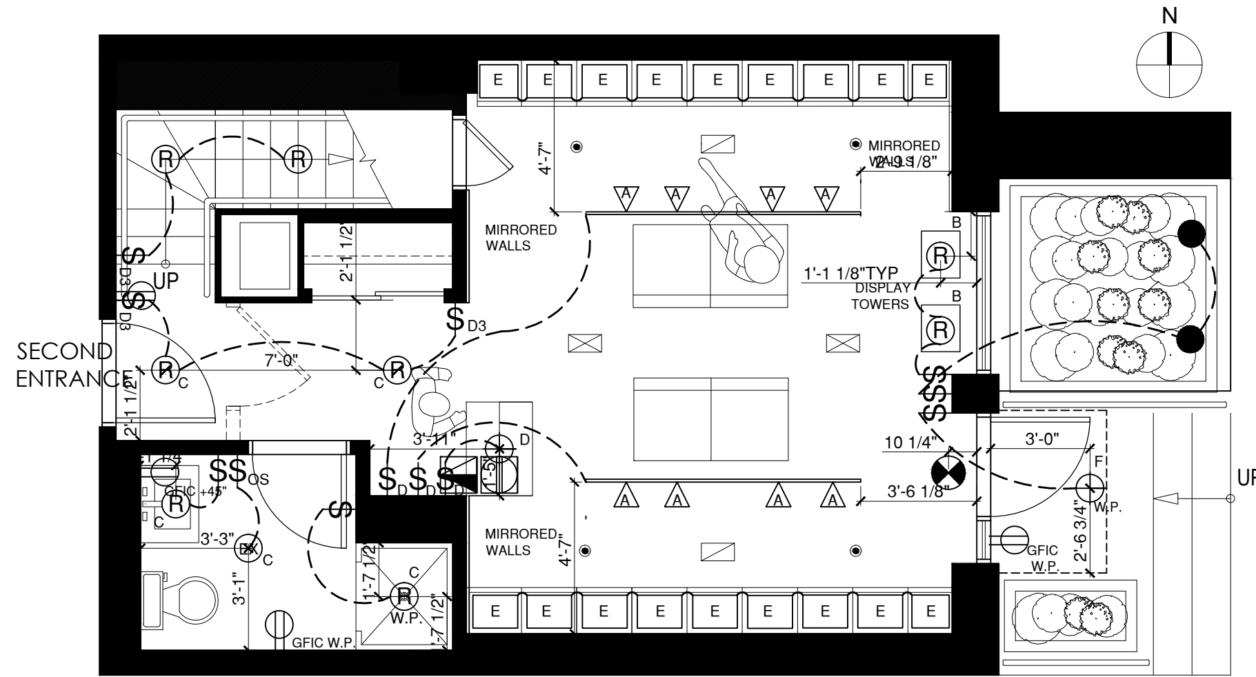
1 GROUND LEVEL PLAN Scale: 1/4"=1'-0"
